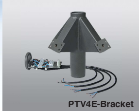
PTV4E-Bracket
